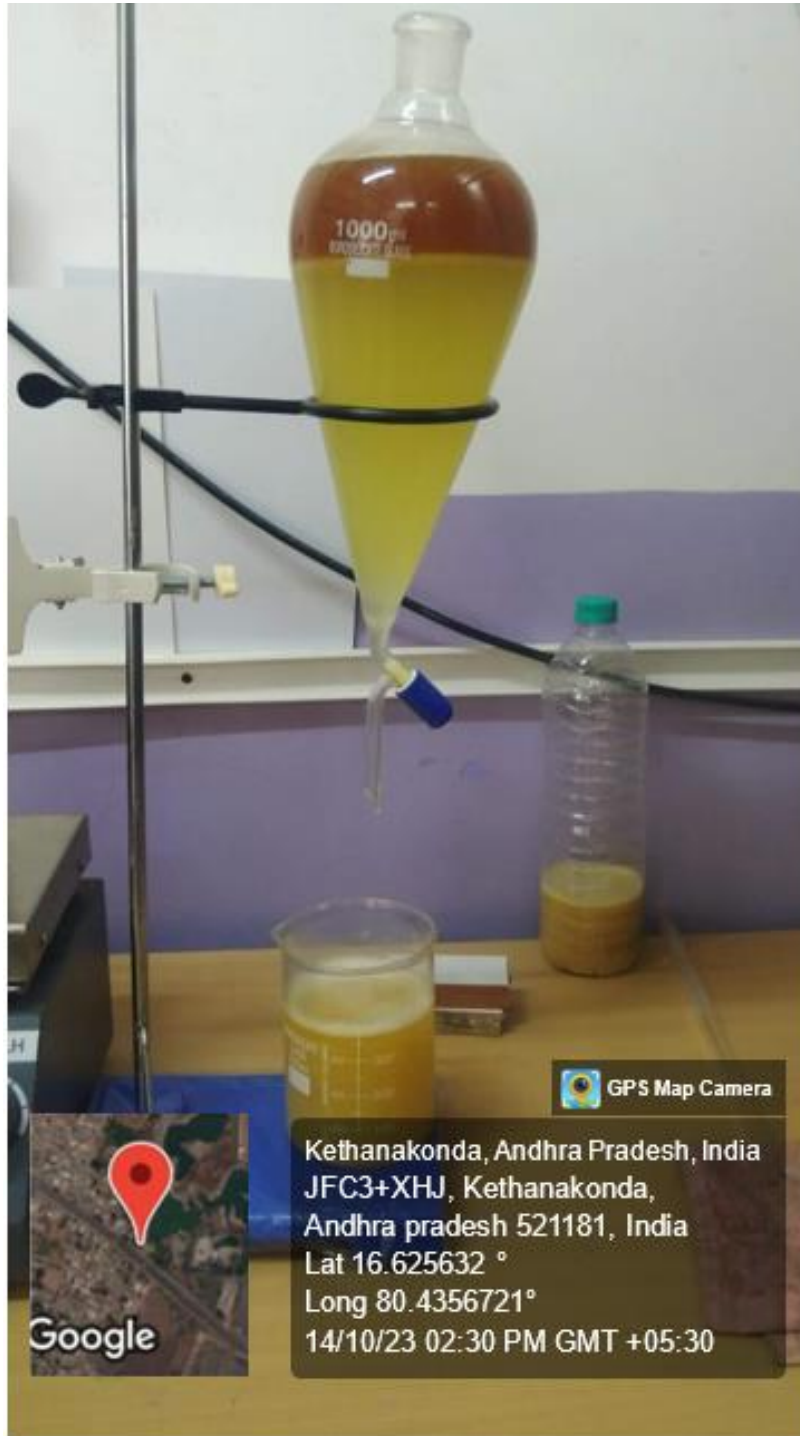
Separating Funnel
